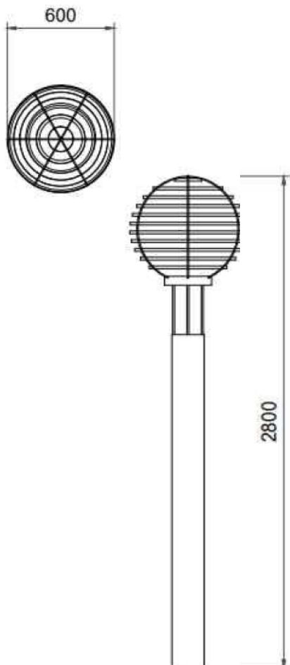
Dimensions Drawing
