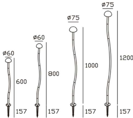
Dimensions Drawing
