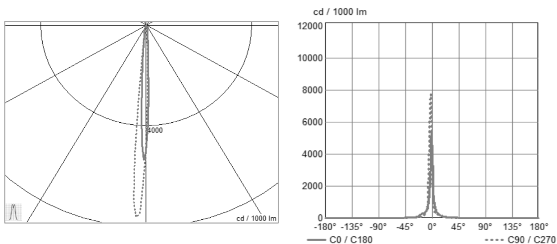
Photometric Data
