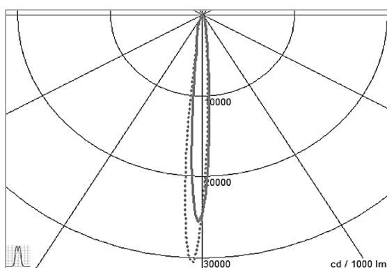
Photometric Data
