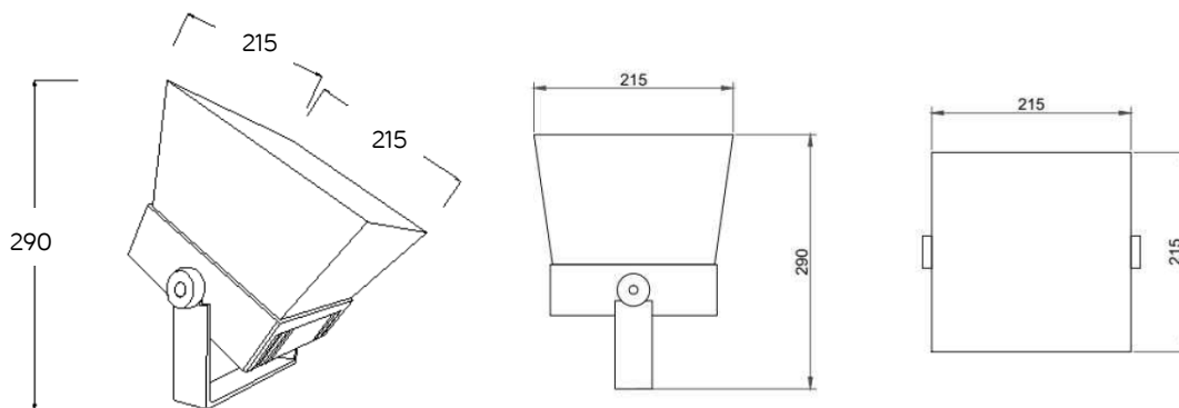
Dimensions Drawing
