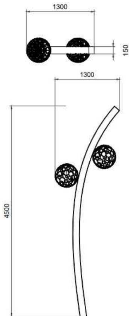
Dimensions Drawing
