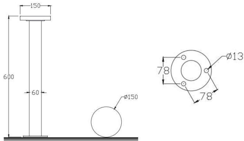
Dimensions Drawing
