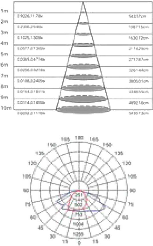
Photometric Data
