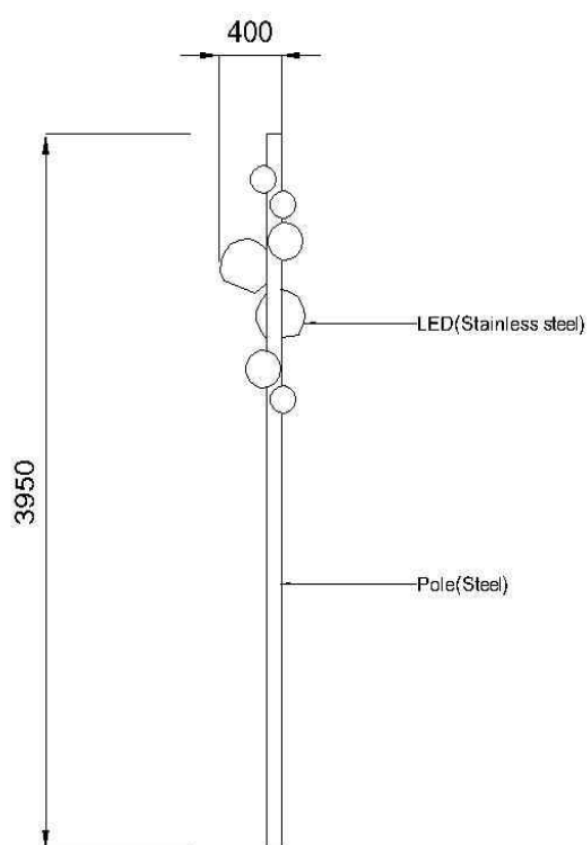
Dimensions Drawing
