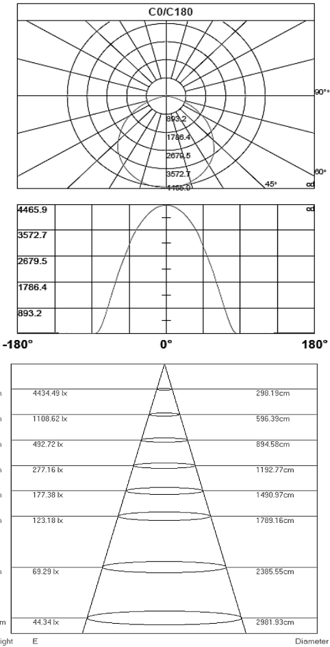
Photometric Data
