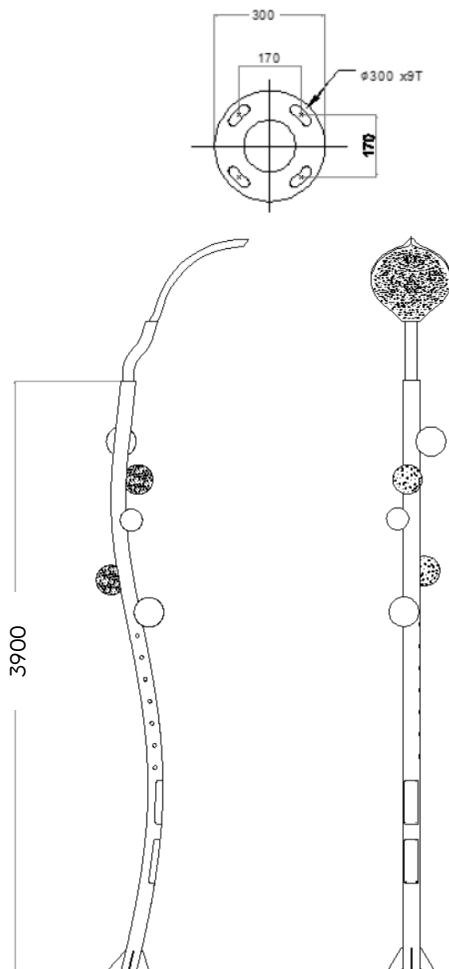
Dimensions Drawing
