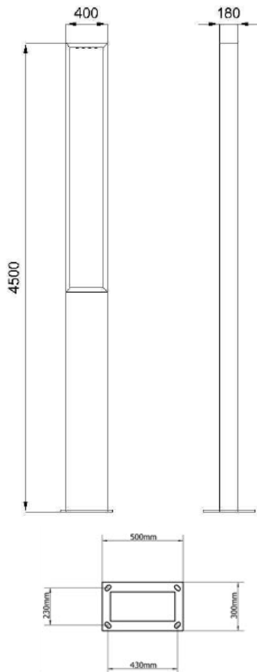
Dimensions Drawing
