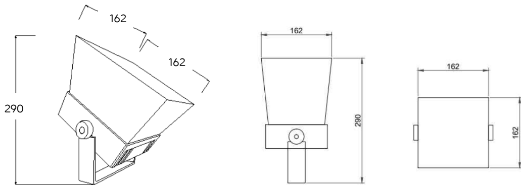
Dimensions Drawing
