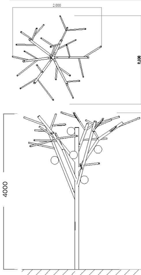
Dimensions Drawing
