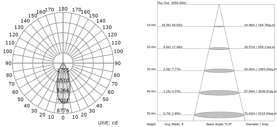
Photometric Data
