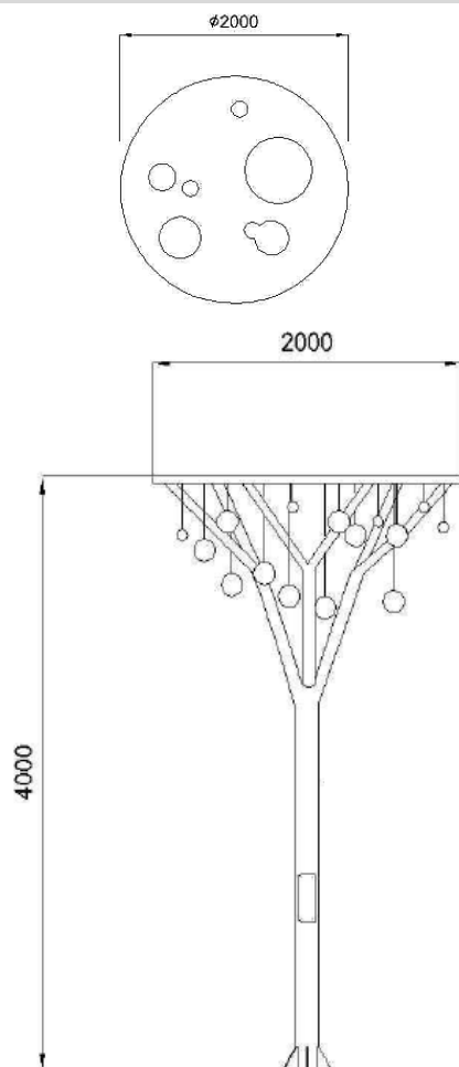
Dimensions Drawing
