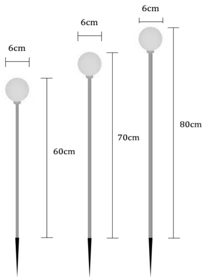
Dimensions Drawing
