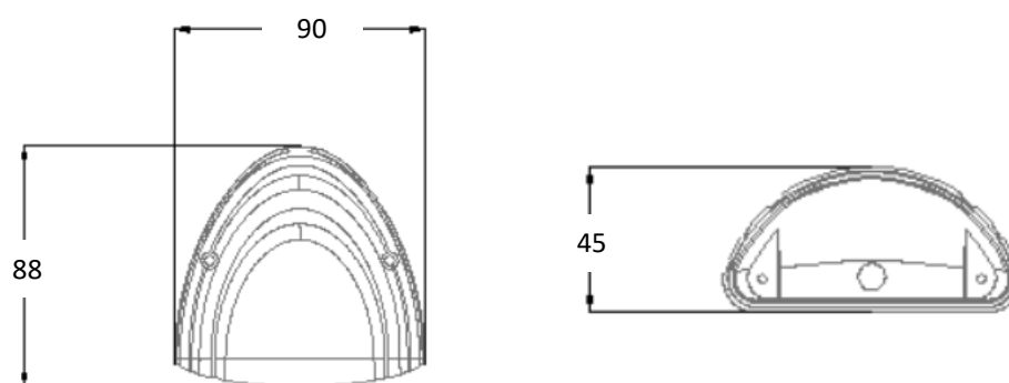
Dimensions Drawing
