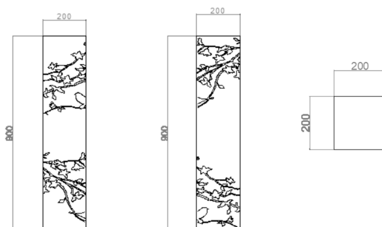
Dimensions Drawing
