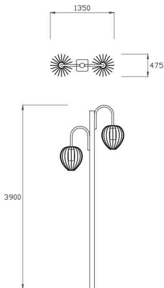
Dimensions Drawing
