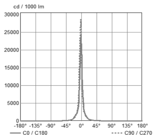
Photometric Data
