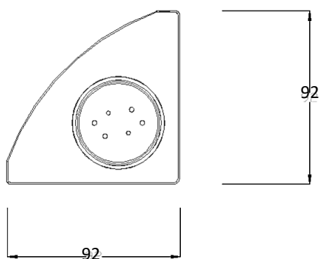
Dimensions Drawing
