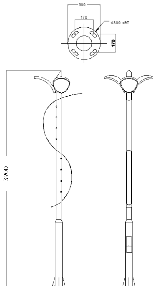
Dimensions Drawing
