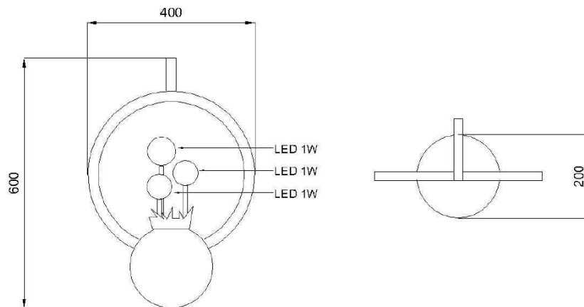
Dimensions Drawing
