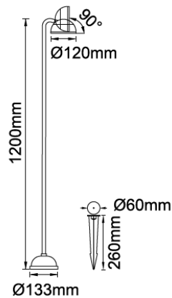
Dimensions Drawing
