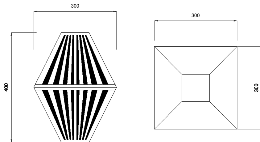
Dimensions Drawing
