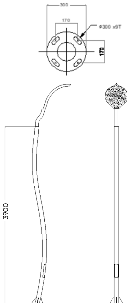
Dimensions Drawing
