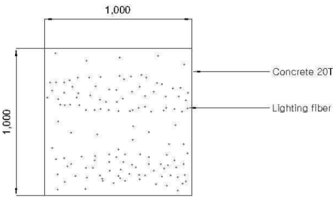
Dimensions Drawing
