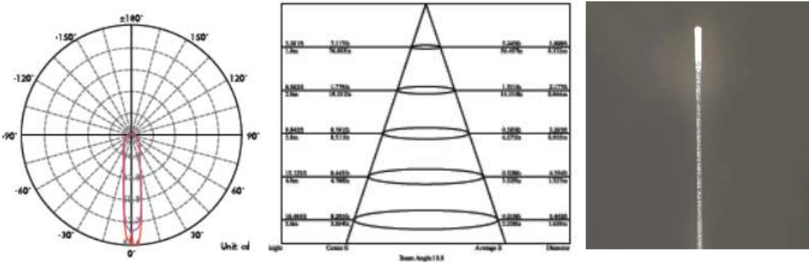
Photometric Data
