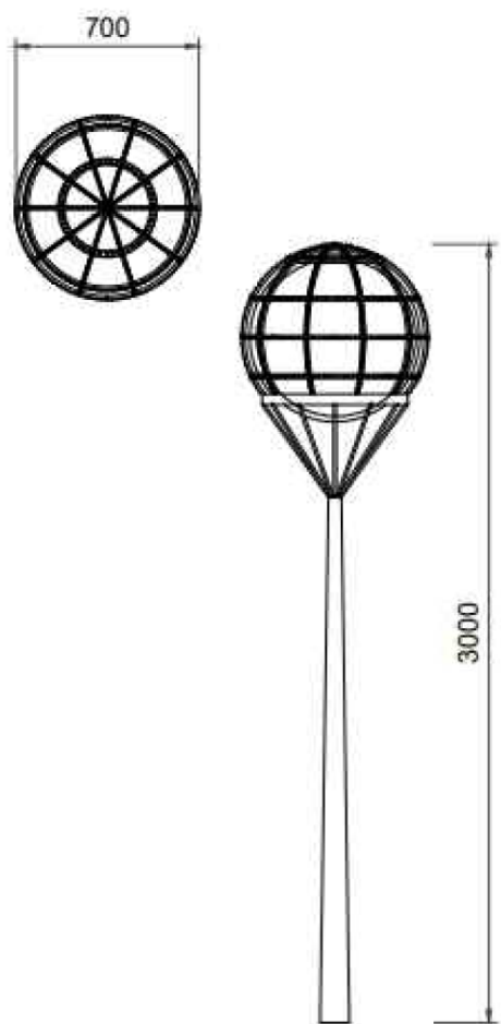
Dimensions Drawing
