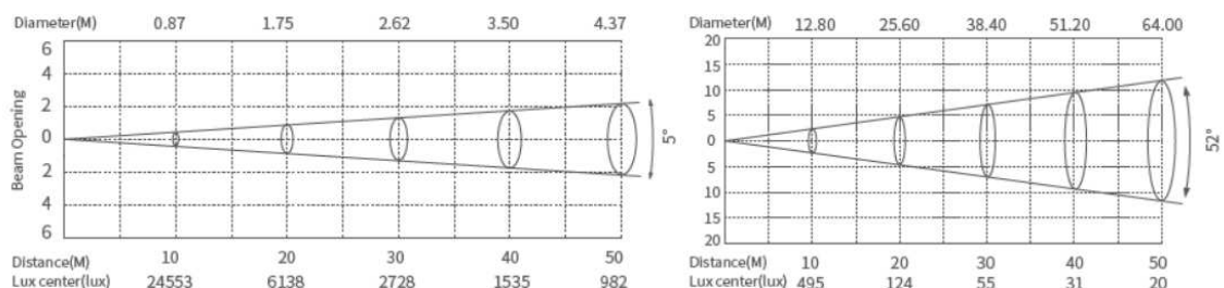
Illuminance at Distance
