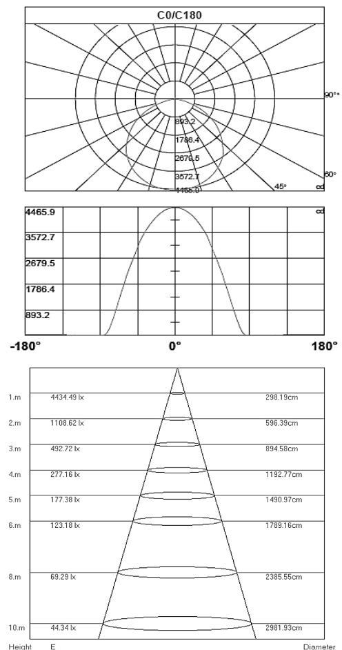
Photometric Data
