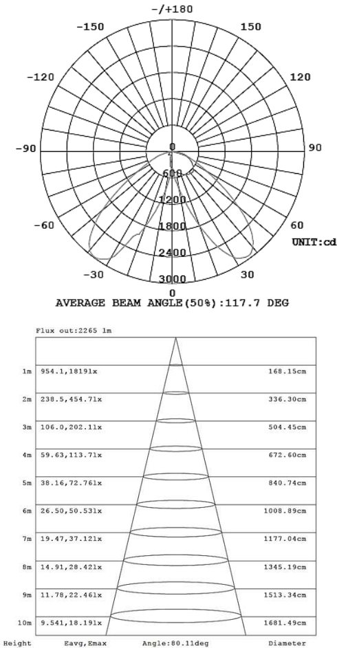
Photometric Data
