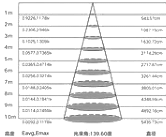
Photometric Data
