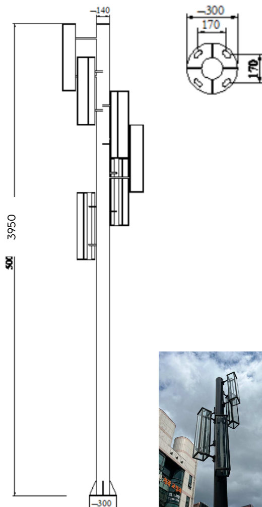
Dimensions Drawing
